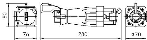
8575/14 Coupler 16 A
